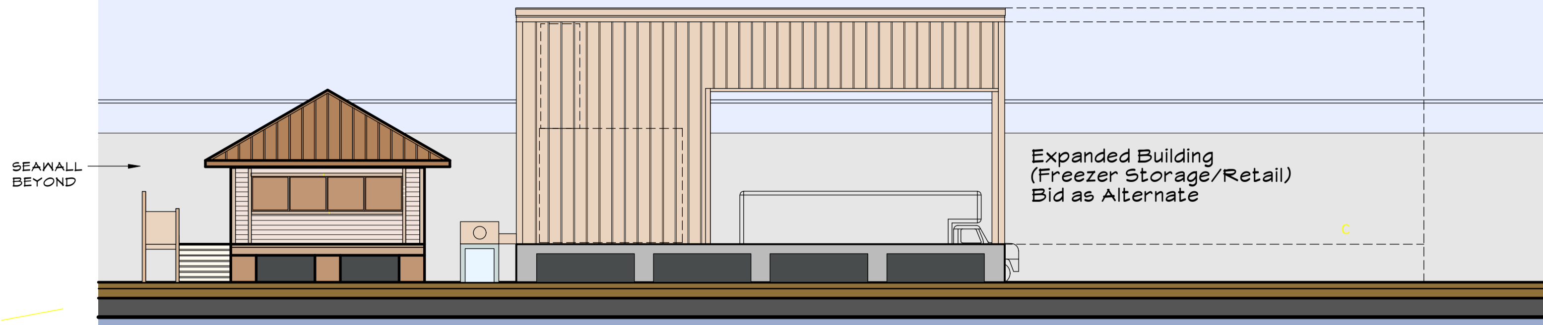
ICE HOUSE OFFICE AND ICE PRODUCTION BUILDING RIVER SIDE ELEVATION 608 SF
